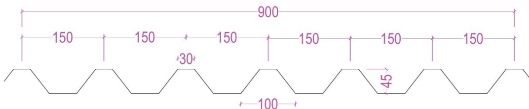
Decking Sheet YX45-/150-900
